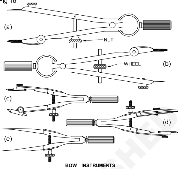
BOW - INSTRUMENTS
