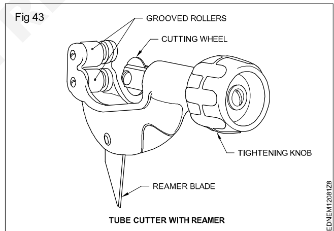
Tube cutter with reamer (Fig 43)
